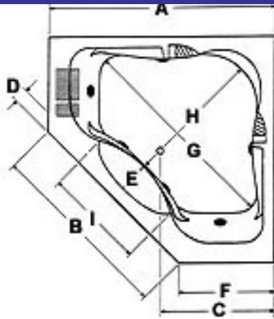
Tub must be set in Mortar Base
